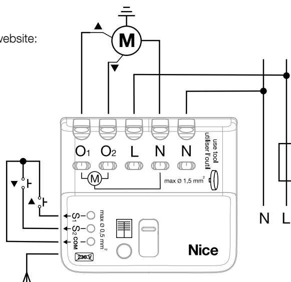
Figure 2: Wiring diagram of BiDi-MiniShutter
